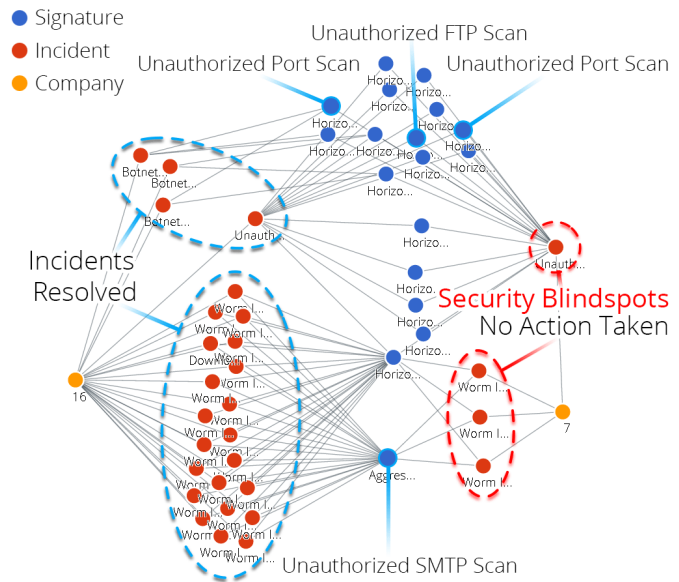
Fig. 13. Results of our first blindspot detection query (see Figure 12A). VIGOR identifies Company 7’s blindspots with evidence that Company 16 is faced with similar security incidents and takes them seriously.
